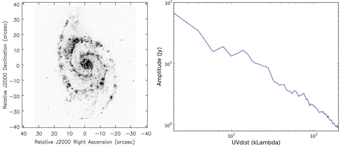
Figure 7.13: Image of H\alpha emission from M51 used as a model of emission at 100 GHz ( left ) and the expected visibility amplitudes (logarithmic scale) plotted versus uv distance ( right ). Note that M51 cannot be observed from ALMA.
