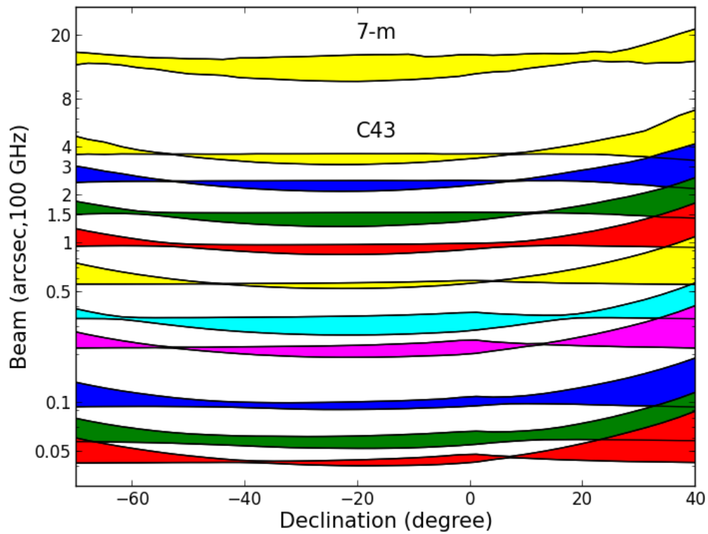
Figure 7.8: Cycle 8 angular resolutions as a function of source declination. Each stripe shows, for a particular notional configuration, the range of the major and minor axes of the synthesized beams expected from a 2-hour observation at 100 GHz and at transit, imaged with robust = 0.5. The notional 12-m Array configurations are arranged with C43-1 at the top and C43-10 at the bottom.
