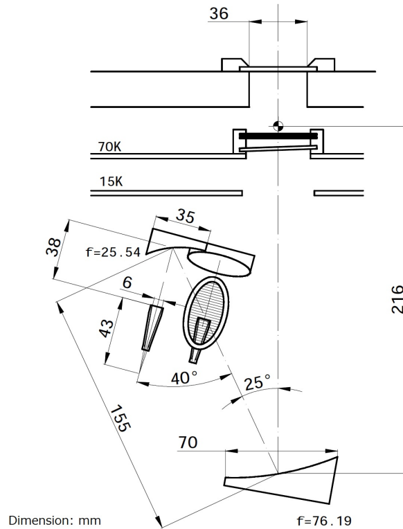
Figure 4.20: Band 7 cold optics arrangement, showing the off-axis ellipsoidal mirrors and the polarization splitter wire grid.
