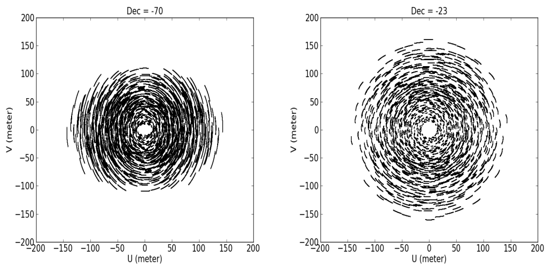
Figure 7.7: uv plane coverage for notional configuration C43-1 with a 1-hour observation of a transiting source at a declination of either -70^\circ (left) or -23^\circ (right). For the source with a declination of -70^\circ , 25.7% of visibilities are expected to be flagged due to shadowing.
