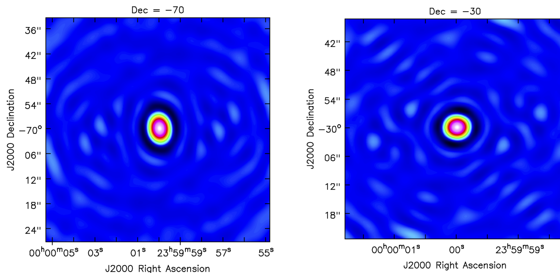
Figure 7.6: Beam shape for notional configuration C43-1 with a 2-hour observation of a transiting source at a declination of either -70^\circ (left) or -30^\circ (right).
