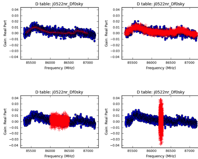
Figure 8.4: A frequency vs real part of the D-terms plot for an antenna (DV22) obtained towards J0522-364. Blue circles and red crosses are showing the D-term obtained using a setup of FDM with 2 GHz bandwidth and using a setup with higher spectral resolutions (FDM 500 and 62.5 MHz bandwidth respectively). Four panels show the D-terms obtained from the spw 0, 1, 3, 2 (from top left, clockwise).
